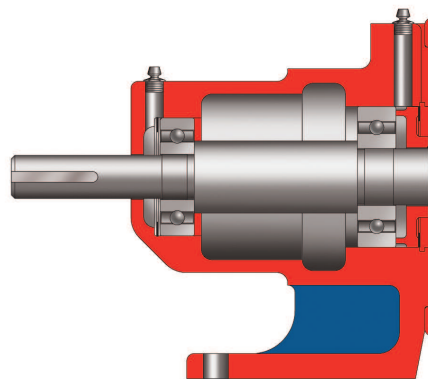
Bearing Frame
